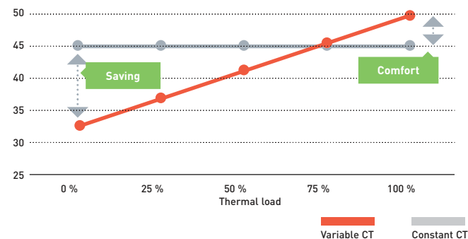
Coolant evaporation temperature (°C)
