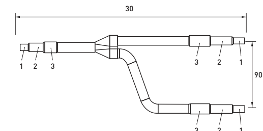
Liquid tubing
