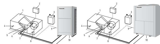
System & regulations. System overview. 1. AHU Unit equipment (field supplied) 2. AHU Unit system controller field supplied 3. AHU Kit controller box (with control PCB) 4. Thermistor for discharge air 5. Electronic expansion valve 6. Thermistor for gas pipe (E3)
