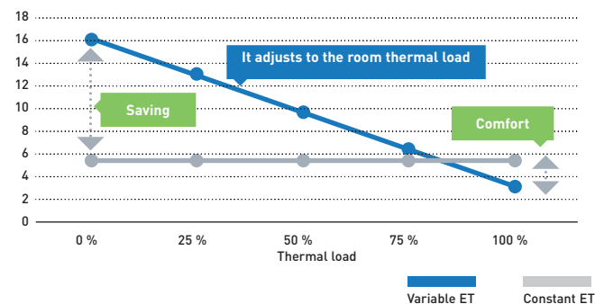
Example of cooling mode (heating mode is also available)
