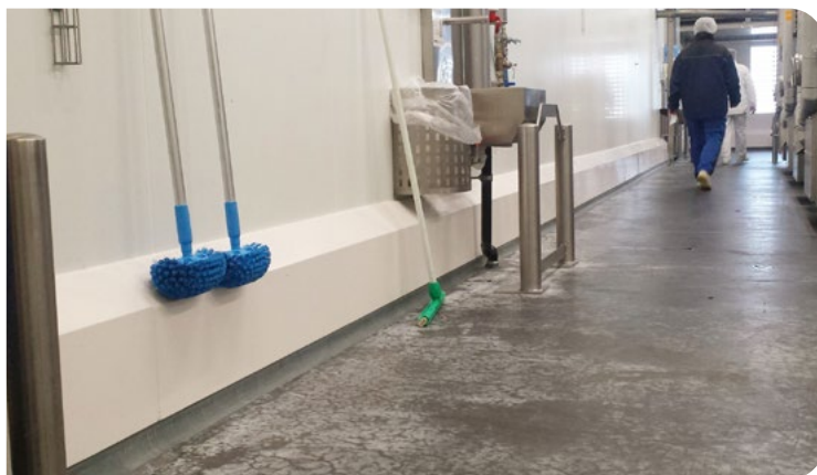
PolySto prefabricated IP40RB Natural CleanRock kerb with a resin floor applied into the rebate.
