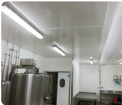
FRP smooth RenoPanel as hygienic ceiling in a dairy processing facility.
