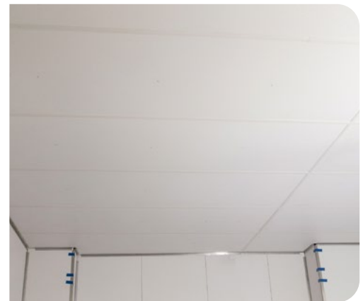
FRP embossed RenoPanel as hygienic ceiling in a meat processing facility.
