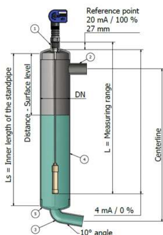
Standpipe: DN65...DN100. Recommended pipe standard: DIN 10220 Recommended bending: DIN 2615-1/ Type 3 Site pipe can be designed in smaller pipe e.g. 0.5 x DN.
