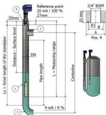
Stand pipe: DN32.....DN65. Recommended pipe standard: DIN 10220 Recommended bending: DIN 2615-1/Type 3 Recommended TEE: DIN 2615-1
