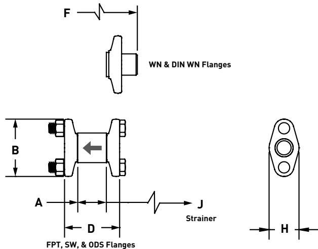
Dimensional Diagram: CK4A Check Valves
