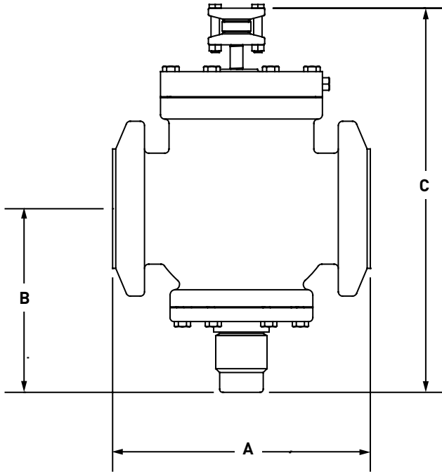
Dimensional Diagram: CK-2 Gas Powered Suction Stop Valves
