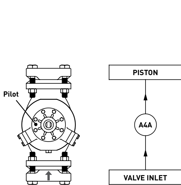
Flow Diagram: A4_Z Inlet Pressure Regulator
