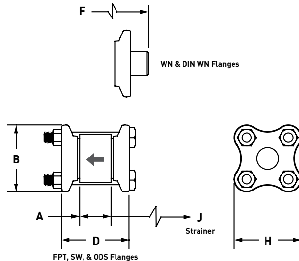
Dimensional Diagram: CK4A Check Valves
