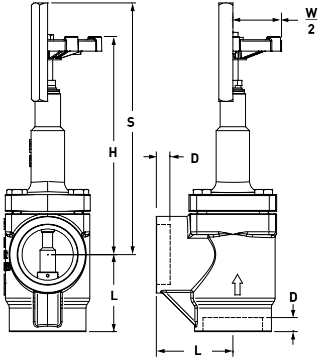
Dimensional Diagram: SW Extended Bonnet Angle Body
