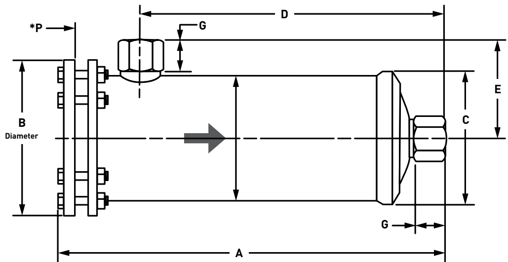
Dimensional Diagram: Core Filter Dryer
